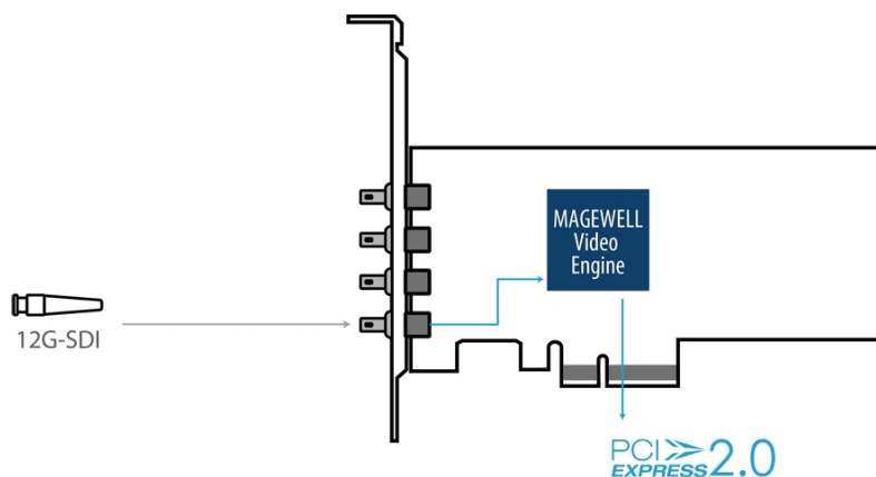
Single-link 12G-SDI
