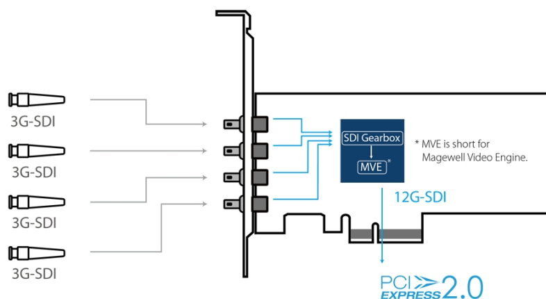
Quad-link 3G-SDI
